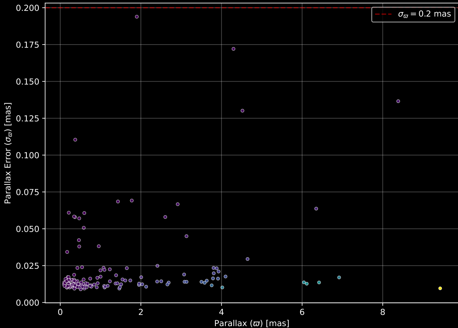
APOGEE DR17 Field: [N2243] Parallax Quality (n= 153)
