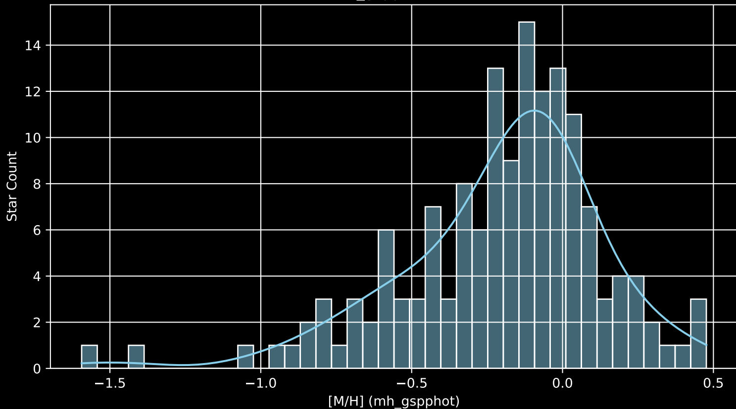
APOGEE DR17 Field: [N2243 [M/H] (mh_gspphot) (n= 150)
