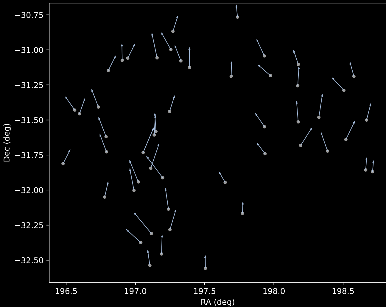
APOGEE DR17 Cluster 1 Proper Motion Vectors (n=50)
