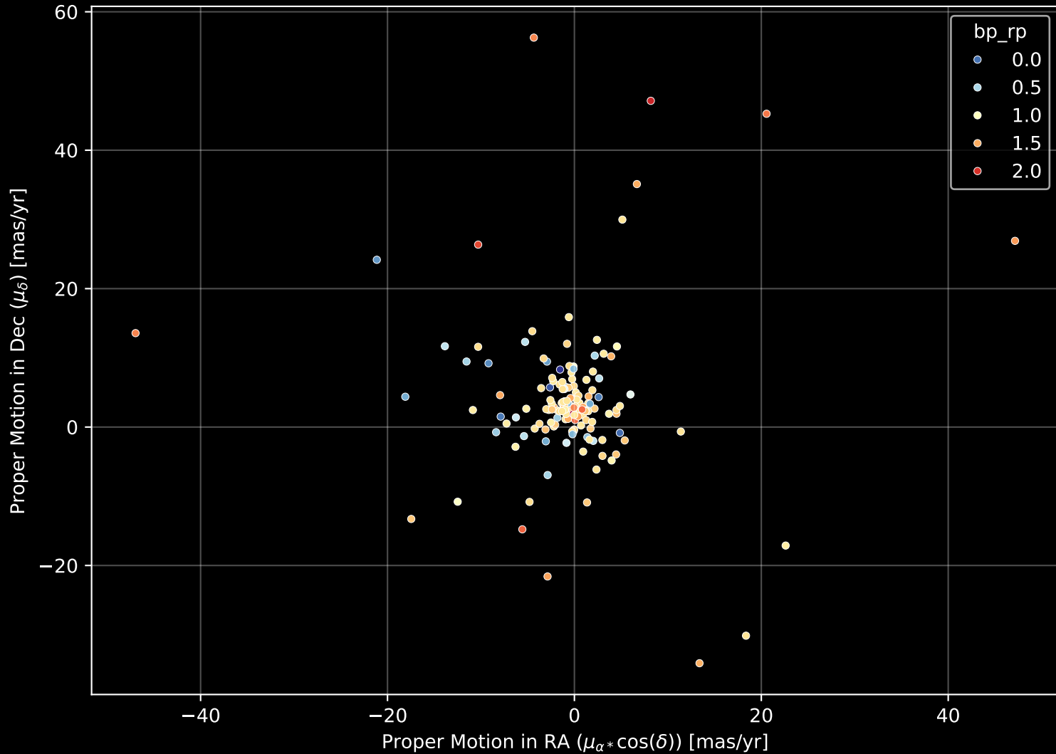
APOGEE DR17 Field: [N2243] Proper Motion Diagram (n= 153)
