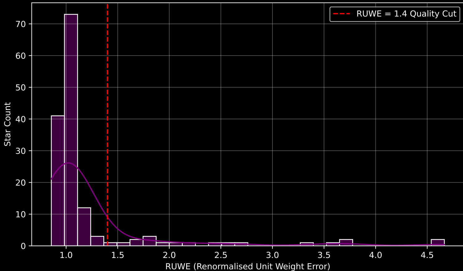
GAPOGEE DR17 Field [N2243] RUWE Distribution (n= 148)
