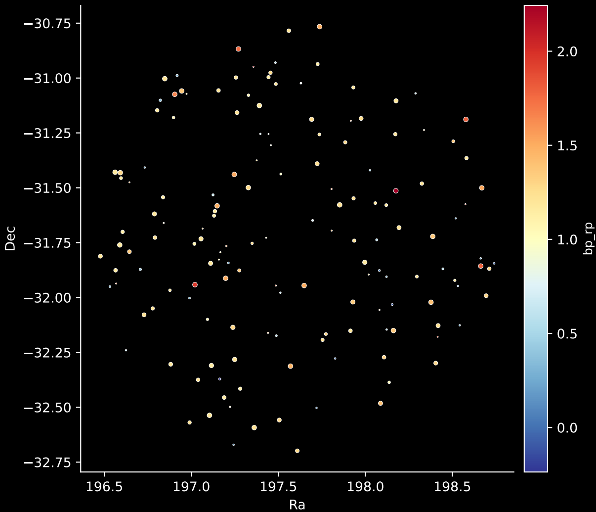
APOGEE DR17 Field: [N2243] Stars: 153
