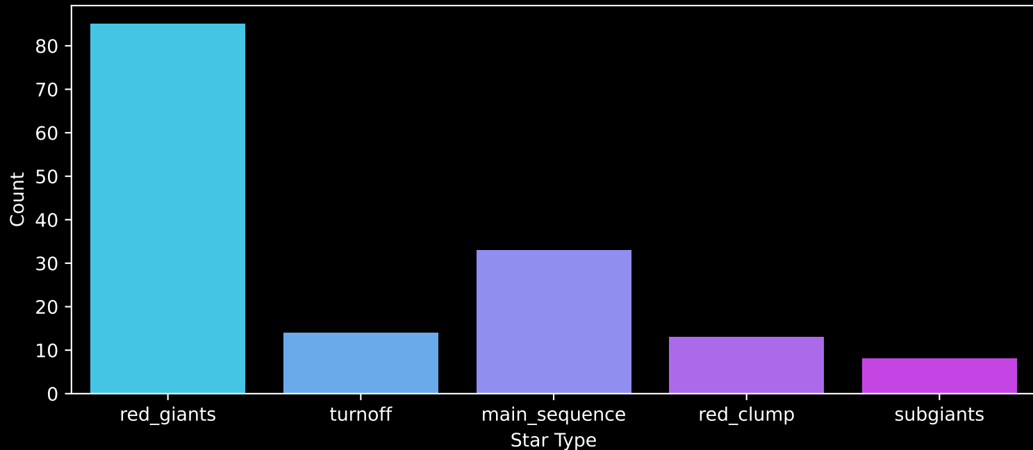
APOGEE DR17 Field: [N2243] Count plot of Star Type
